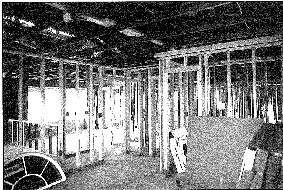
Figure 30 Interior partition walls and utilities are added.
