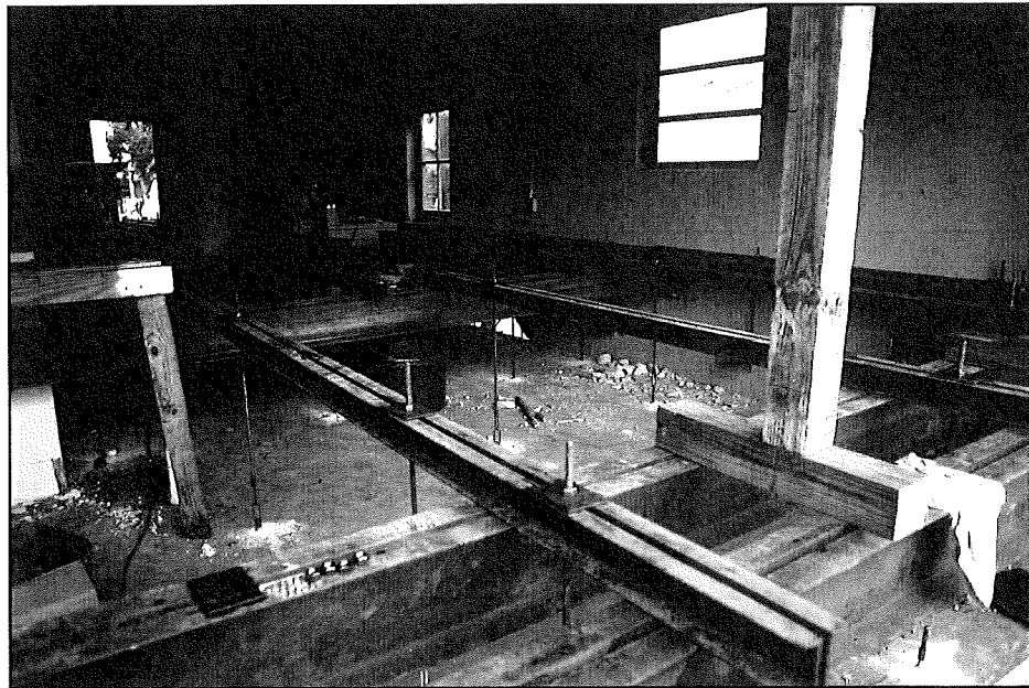
Figure 79 The anchors and hangers connect the slab securely to the beams, enabling the beams to raise the slab along with the rest of the house.
