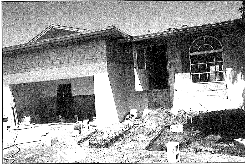
Figure 29 Windows and doors are added. The height of the raised front door shows the amount of elevation.
