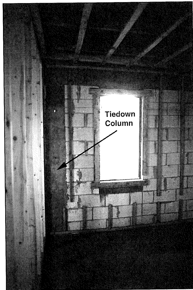
Figure 46 Concrete tiedown columns, such as the one to the left of the window in this photograph, were also used in this house.
